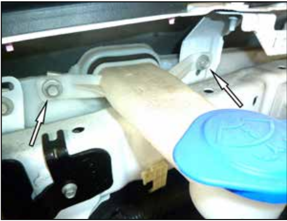
15. Remove the two bolts that secure the washer bottle filler neck to the bottle and remove the neck from the vehicle. NOTE: These parts will be reinstalled.
