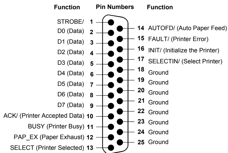
Parallel 25-Pin D-Shell
