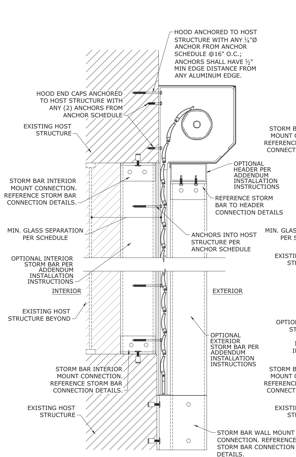
1 WALL MOUNT (SHOWN W/ OPTIONAL STORM BARS)
