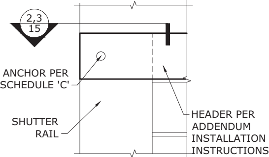
1 15 BUILD-OUT & WALL MOUNT N.T.S. ELEV
