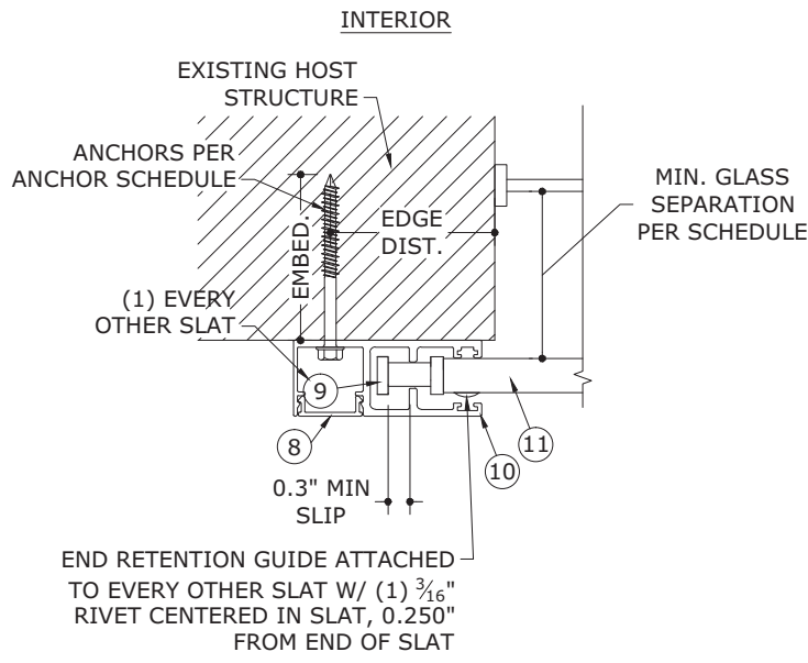
1 4 END RETENTION TYPICAL WALL MOUNT N.T.S. HORIZ SECTION
