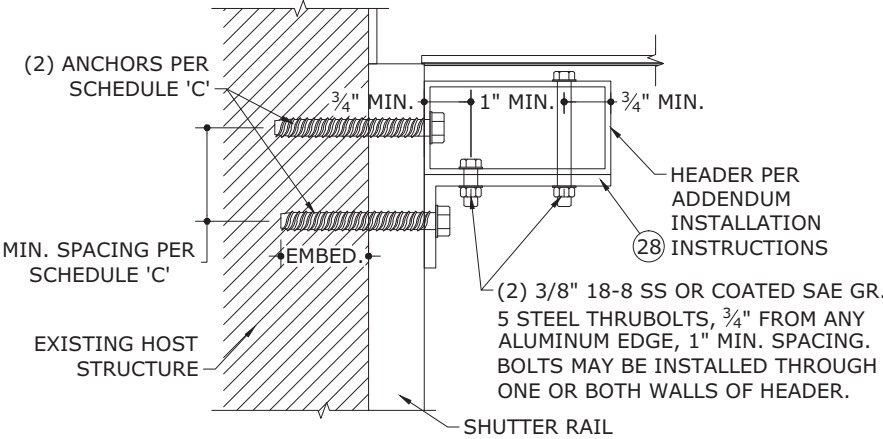
5 15 WALL MOUNT N.T.S. VERT SECTION
