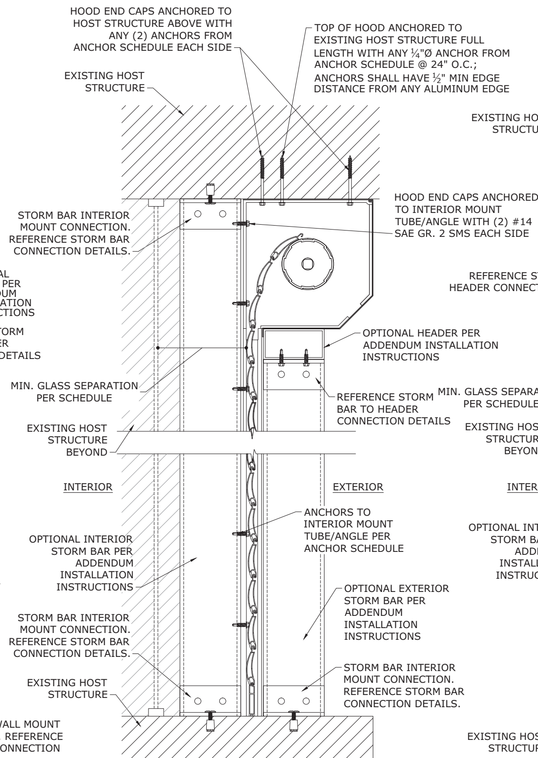
2 INTERIOR MOUNT (SHOWN W/ OPTIONAL STORM BARS)
