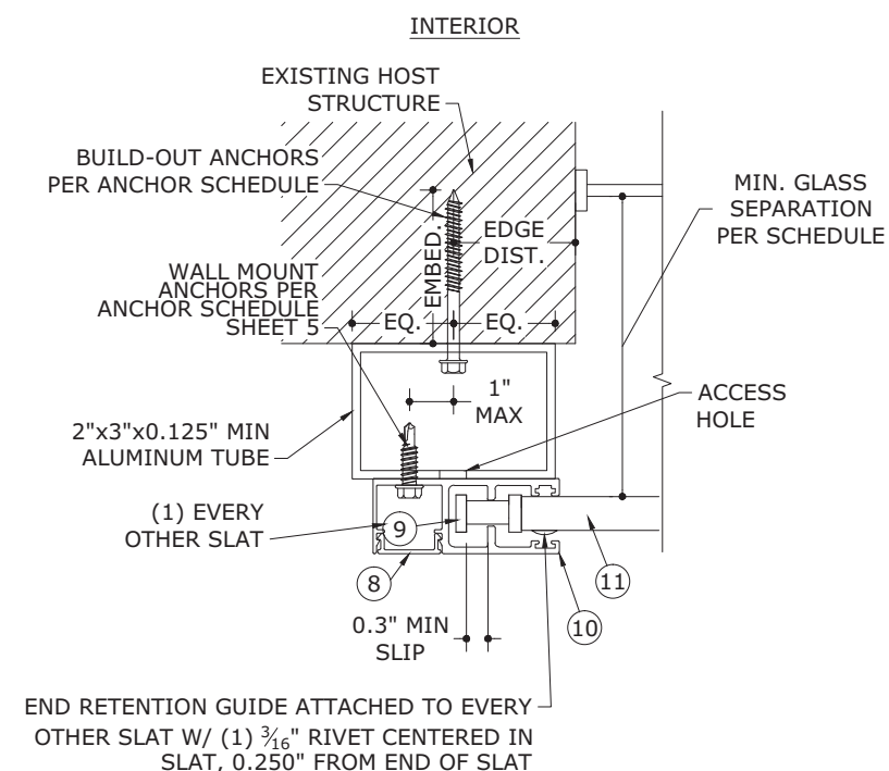
2 4 END RETENTION TYP. BUILD-OUT MOUNT N.T.S. HORIZ SECTION
