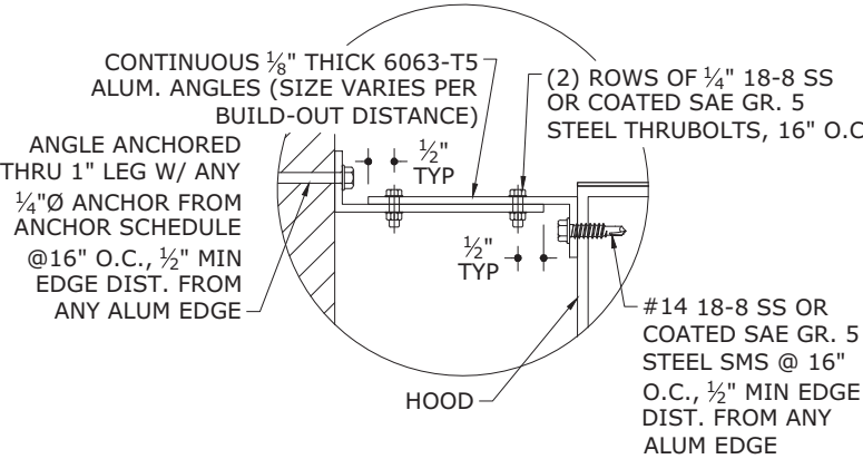
2 11 ALTERNATE BUILD-OUT HOOD CONNECTION SECTION N.T.S.
