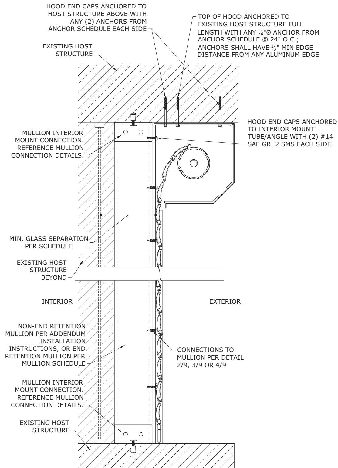
1 MULLION INTERIOR MOUNT 10 N.T.S. VERT SECTION
