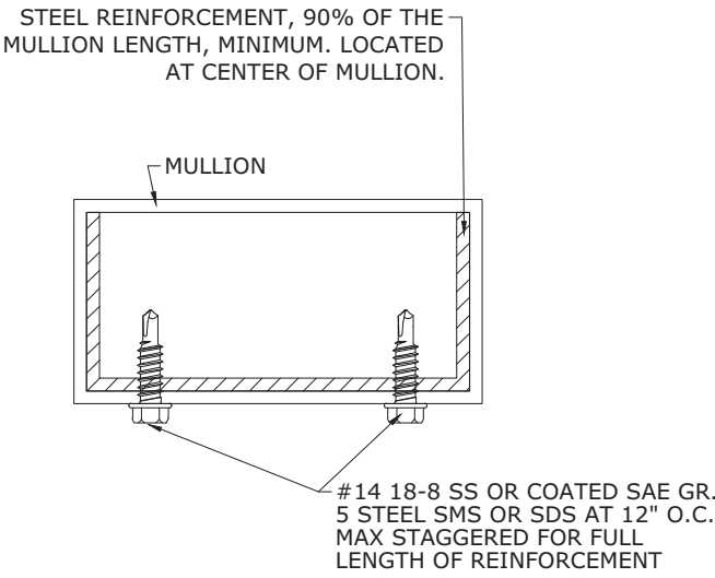
1 11 TYPICAL REINFORCEMENT SECTION N.T.S.
