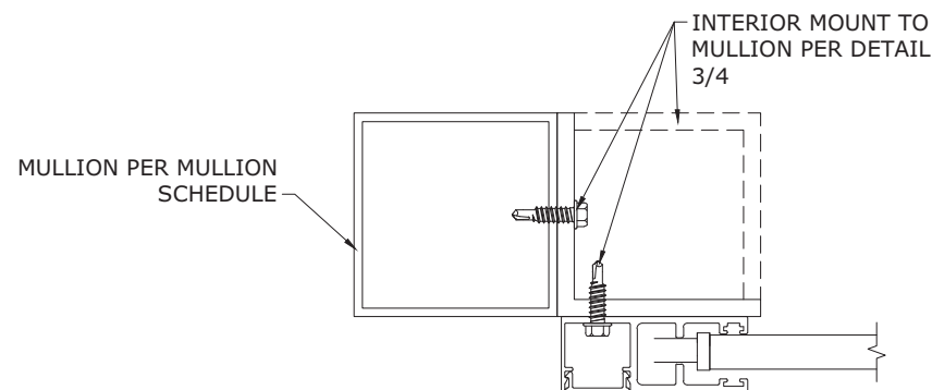
2 9 WALL MOUNT TO INTERMEDIATE MULLION N.T.S. HORIZ SECTION
