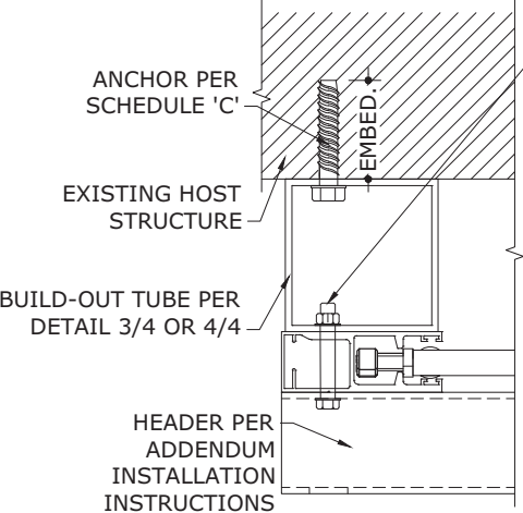
3 15 BUILD-OUT MOUNT N.T.S. HORIZ SECTION
