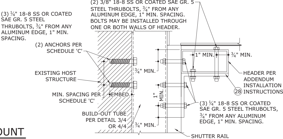
6 15 BUILD-OUT MOUNT N.T.S. VERT SECTION
