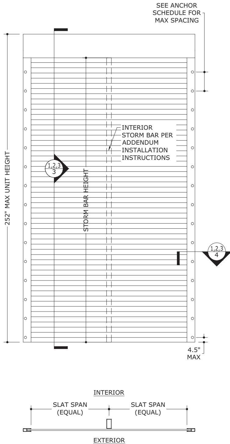
1 8 END RETENTION SHUTTER WITH INTERIOR STORM BARS (DOUBLE-SPAN) N.T.S. EXTERIOR ELEV
