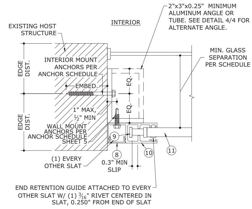
3 4 END RETENTION TYP. INTERIOR MOUNT N.T.S. HORIZ SECTION
