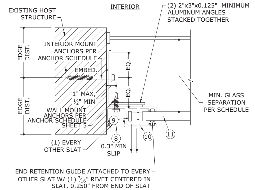
4 4 END RETENTION TYP. INTERIOR MOUNT N.T.S. HORIZ SECTION
