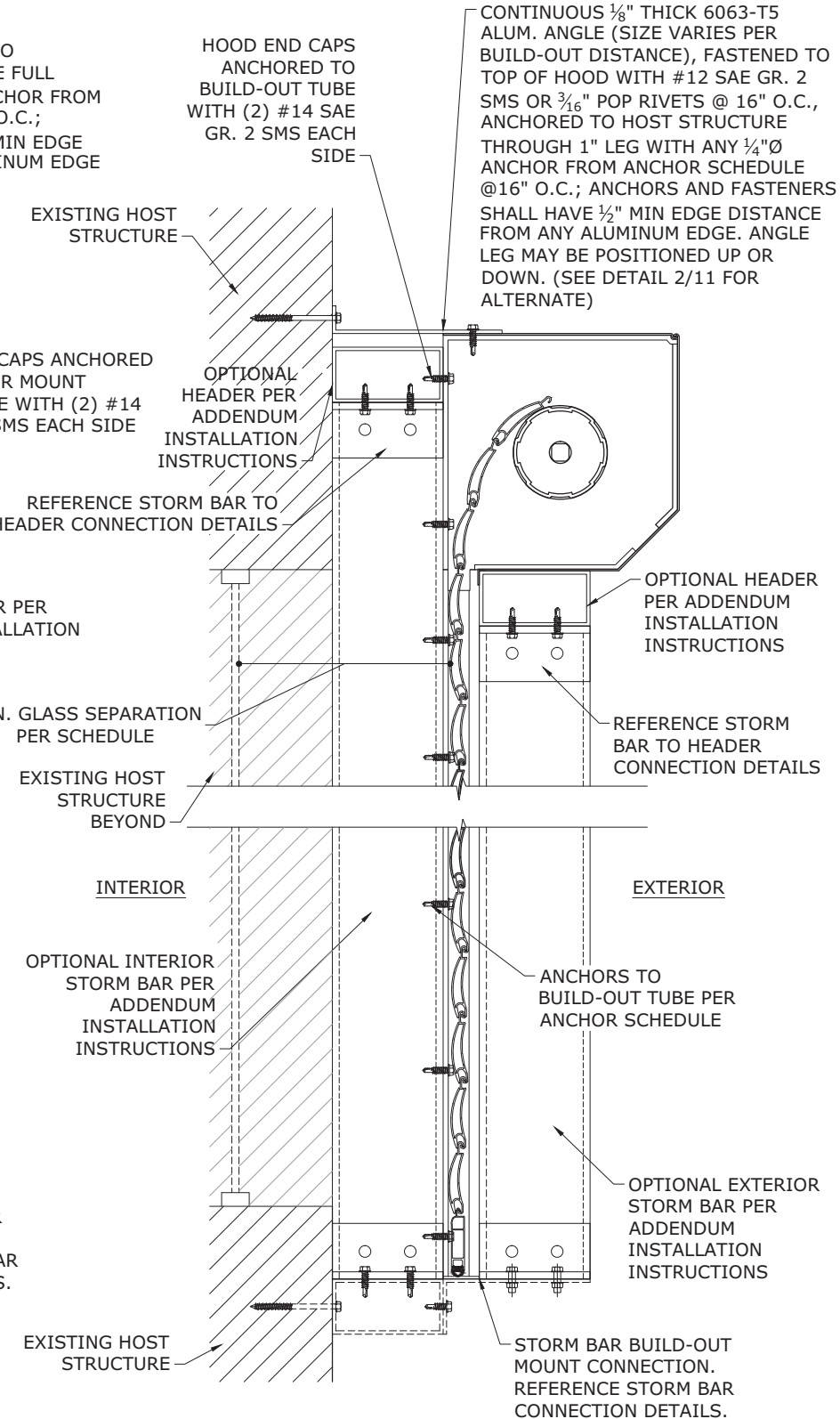
3 BUILD-OUT MOUNT (SHOWN W/ OPTIONAL STORM BARS)
