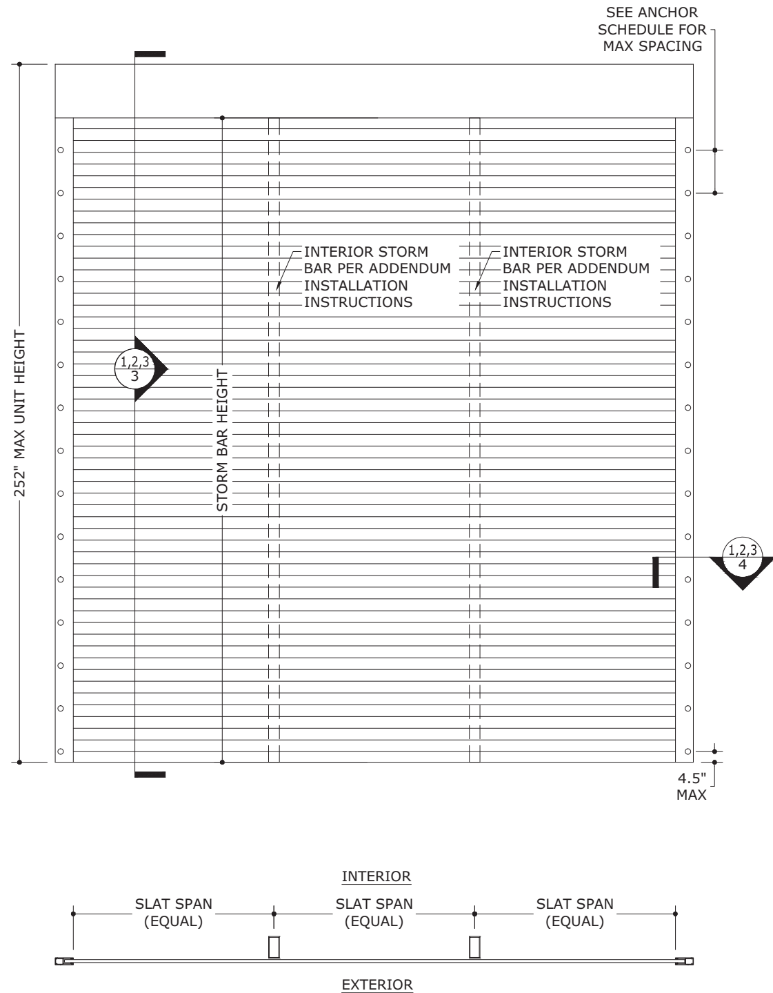
2 8 END RETENTION SHUTTER WITH INTERIOR STORM BARS (TRIPLE-SPAN) N.T.S. EXTERIOR ELEV
