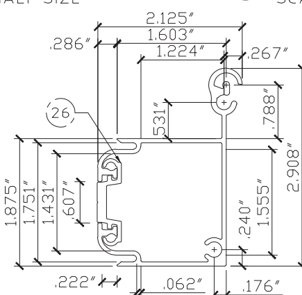
32 FEMALE BOX CENTER SCALE: HALF SIZE
