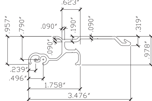
30 UNIMATE LOCK SCALE: HALF SIZE
