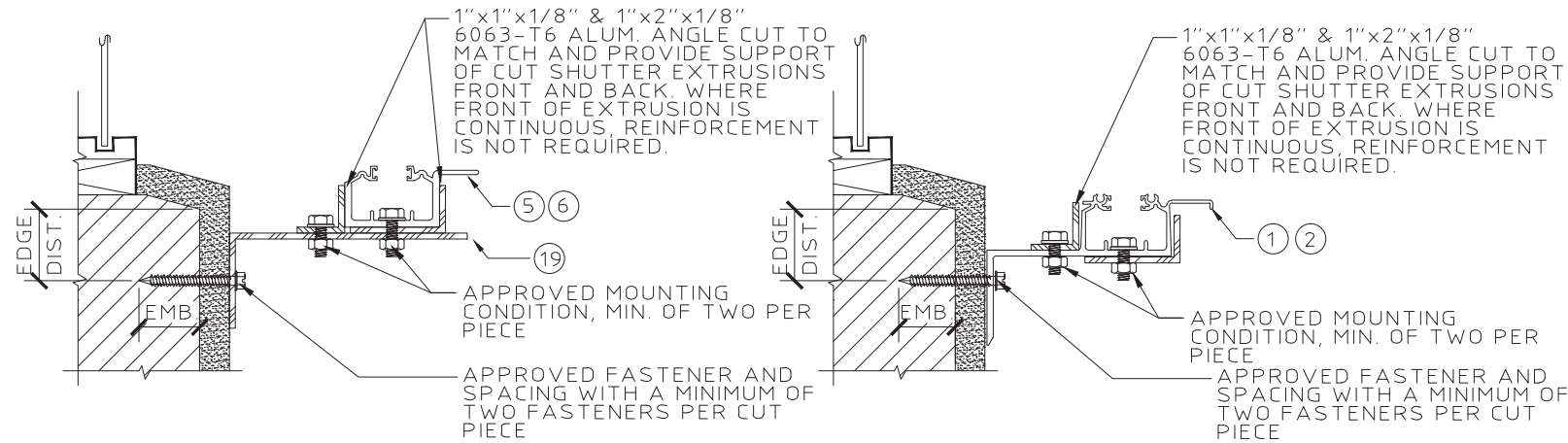
(P1) TYP. SECTION FOR SHUTTERS SCALE: 3" = 1'-0"
