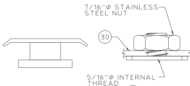
37 T-SCREW INSERT SCALE: FULL SIZE
