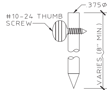
21 SLIDE ROD SCALE: HALF SIZE FOR USE WITH 33 AND 34 ONLY
