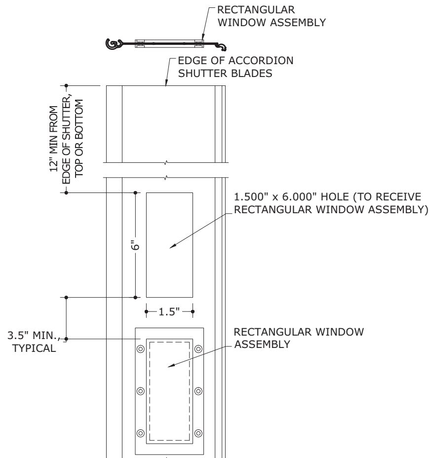
4 BLADE W/ RECT. WINDOW 13 N.T.S. EXTERIOR ELEV
