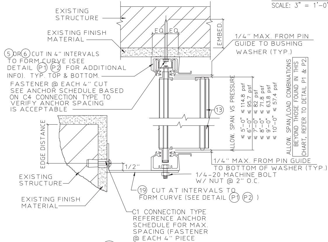
(P) CURVED TRACK SECTION DETAIL SCALE : 3" = 1'- 0"
