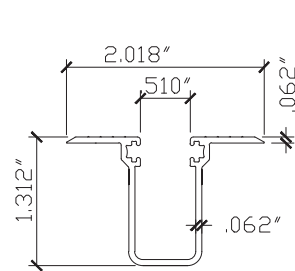
20 RECESS SILL SCALE: HALF SIZE
