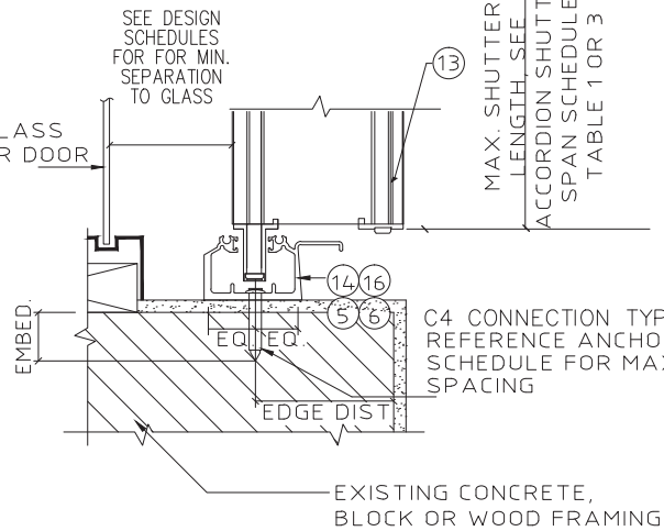
EE INSIDE SILL MOUNT SECTION SCALE: 3" = 1'-0"
