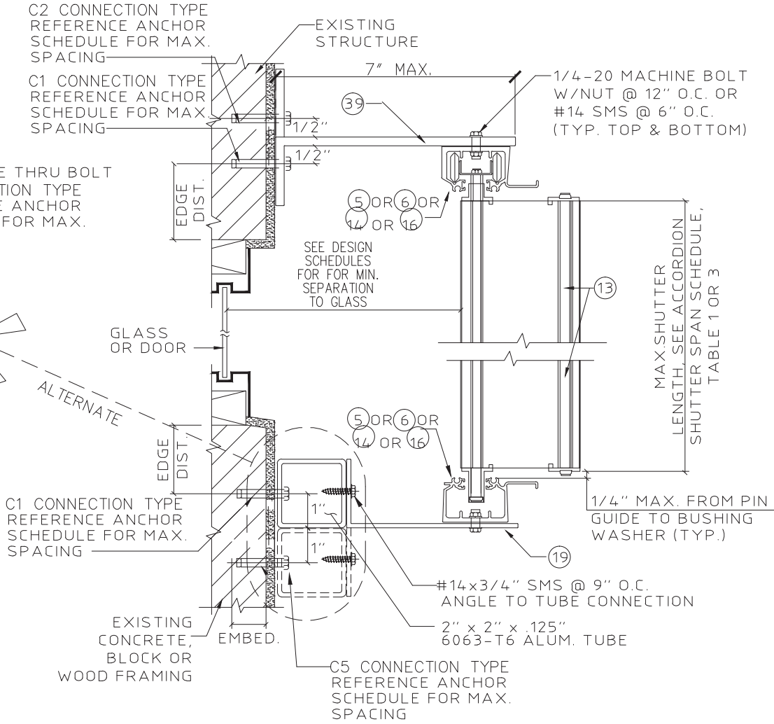
Cb ALTERNATE BUILD OUT MOUNT SECTION SCALE: 3" = 1'-0"
