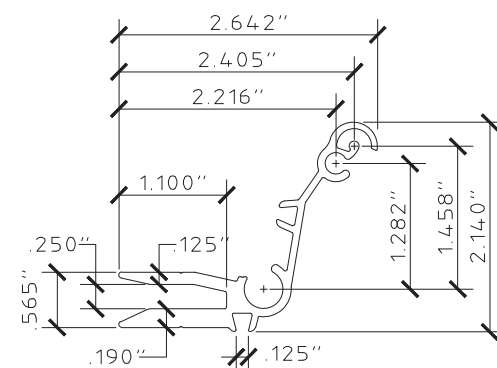
34 INSIDE CENTER MATE SCALE: HALF SIZE
