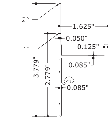
40d ALT. 1" OR 2" END STRIP SCALE: HALF SIZE
