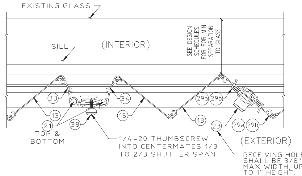
MULTIPLE SHUTTER ASSEMBLY SCALE: 3" = 1'-0"
