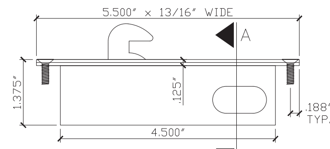
35 BOX LOCK SCALE: HALF SIZE DELTA MODEL 2022 INDUSTRIAL SYSTEMS
