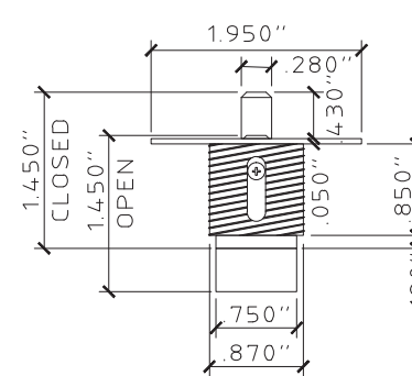
23 BRASS PUSH LOCK SCALE: HALF SIZE CYLINDER-SOLID BRASS, NICKEL PLATED HOUSING-ZINC DICAST, POWDER COATED NOTE: MAY BE KEY OPERATED OUTSIDE OR THUMB TURN OPERATED INSIDE.
