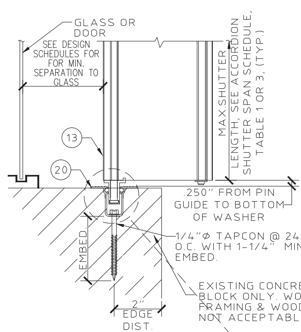
(M) RECESS SILL DETAIL SCALE : 3" = 1'- 0"
