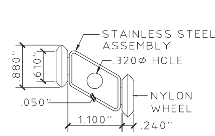
22 ROLLER ASSEMBLY SCALE: HALF SIZE TYP. AT EVERY OTHER INSIDE JOINT AT TOP.
