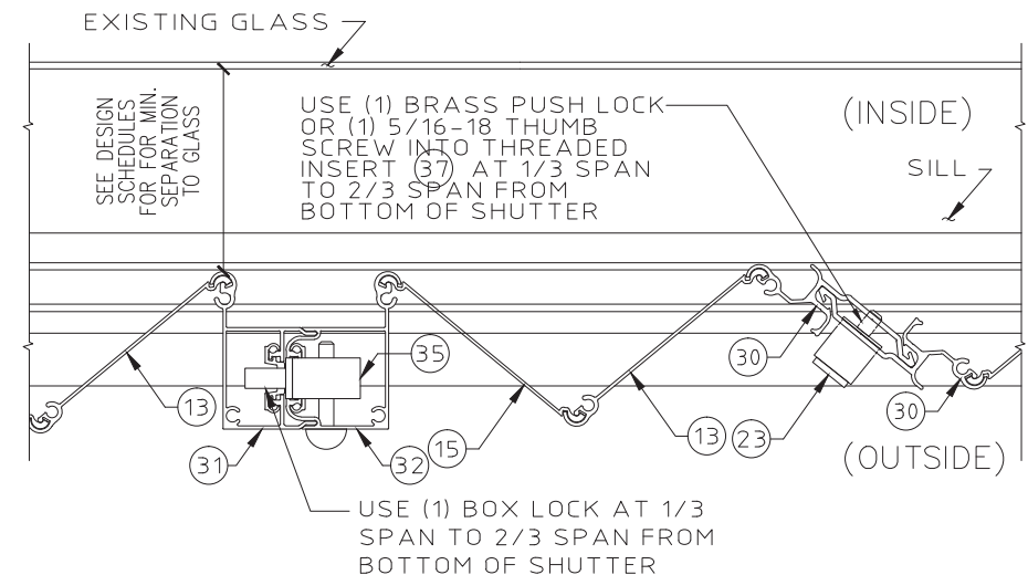
MULTIPLE SHUTTER ASSEMBLY SCALE: 3" = 1'-0"
