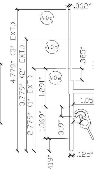
33 OUTSIDE CENTER MATE SCALE: HALF SIZE
