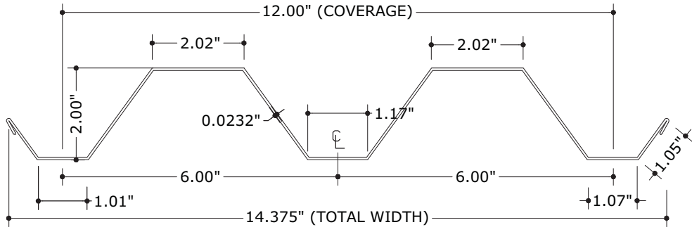
1 STEEL STORM PANEL
