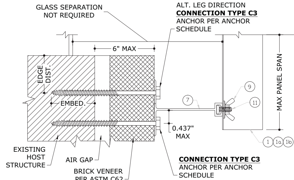
Q BUILD-OUT "F" TRACK THROUGH VENEER OVER STRUCTURAL BASE SECTION
