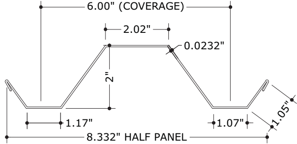
1a STEEL HALF STORM PANEL
