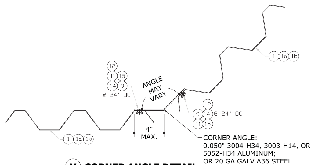
V CORNER ANGLE DETAIL
