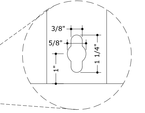
3 KEYHOLE PUNCH 1 6" = 1'-0" ELEV
