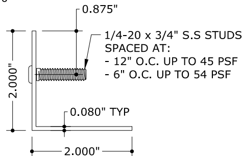
2 STUDDED ANGLE 6" = 1'-0"
