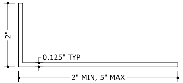
2 STUDDED ANGLE 6" = 1'-0"
