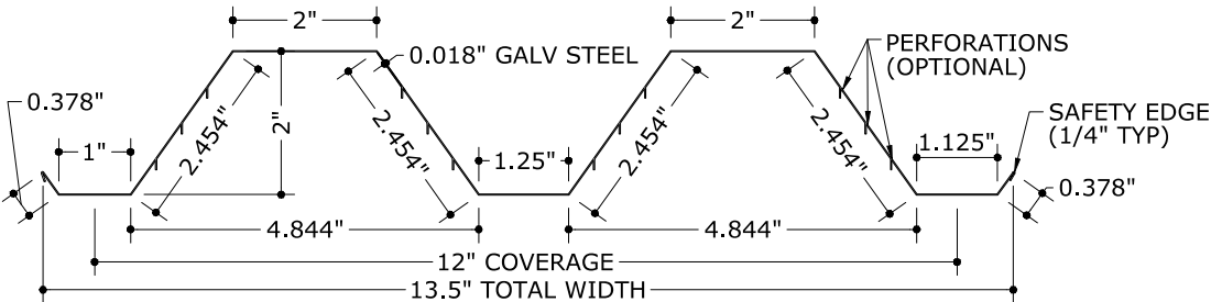
1a STEEL STORM PANEL PROFILE 4" = 1'-0" SECTION
