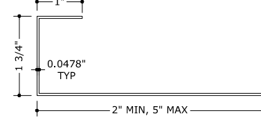
5 STEEL J-PAN CLOSURE 4" = 1'-0"
