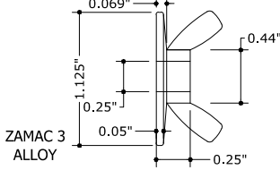
7 WIDE BASE WASHERED WING NUT NTS
