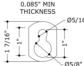
3 KEYHOLE WASHER 6" = 1'-0"
