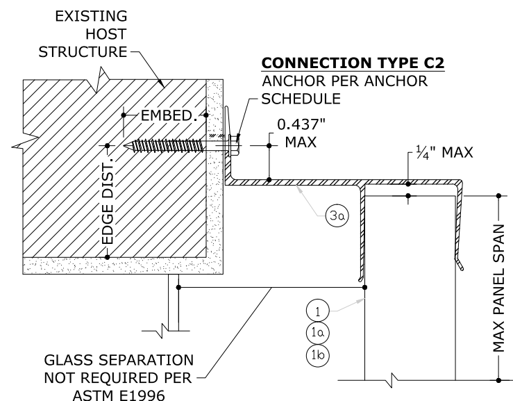
B BUILD-OUT "U" MOUNT SECTION
