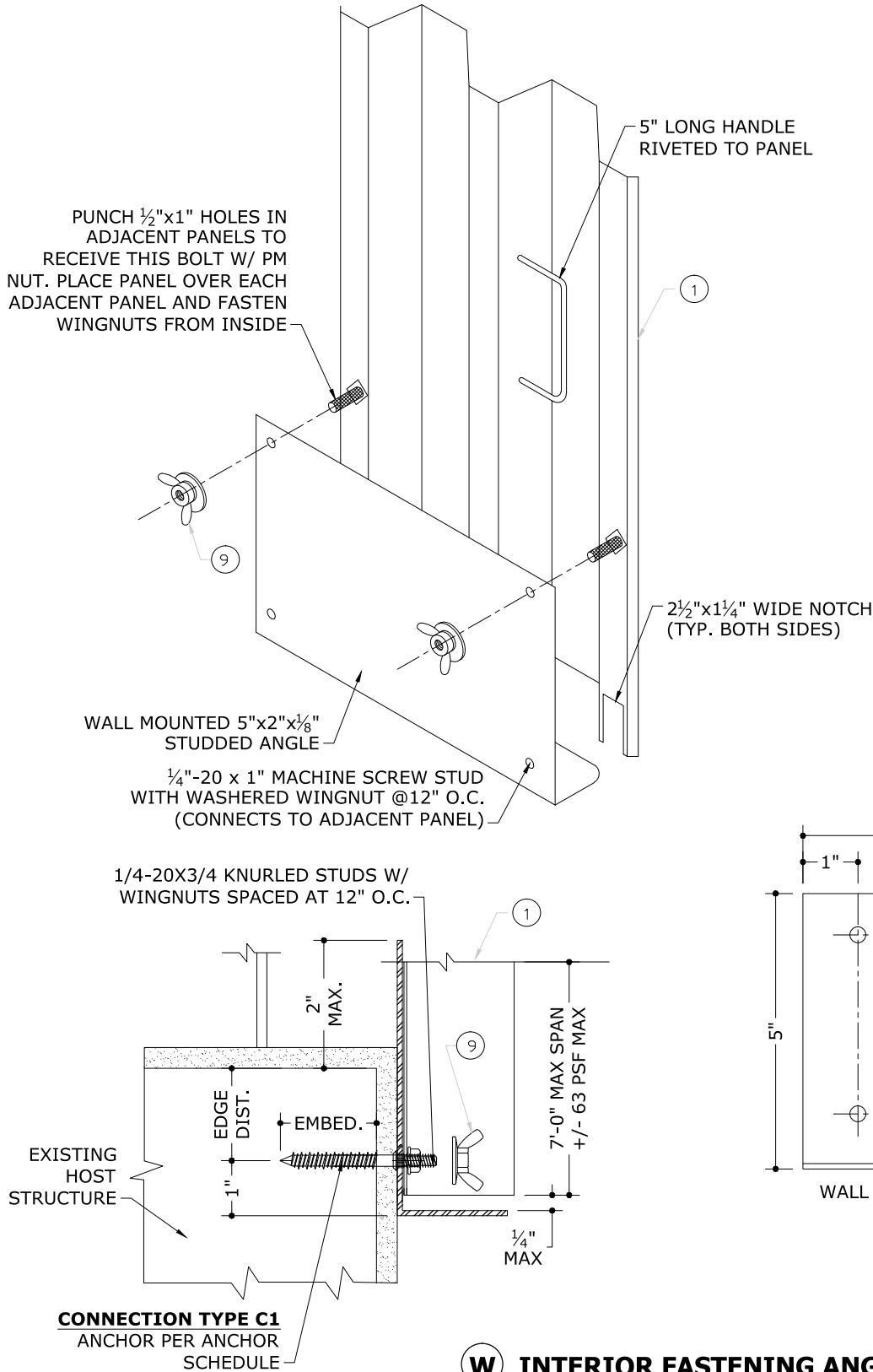
W INTERIOR FASTENING ANGLE ASSEMBLY THESE DETAILS DEPICT THE CONNECTION OF ANY PANEL FOR AN OPENING WITH PANELS INSTALLED FROM INSIDE. USE OF THESE DETAILS SHALL BE IN CONJUNCTION WITH AN "H" HEADER OR "U" HEADER TOP MOUNT.
