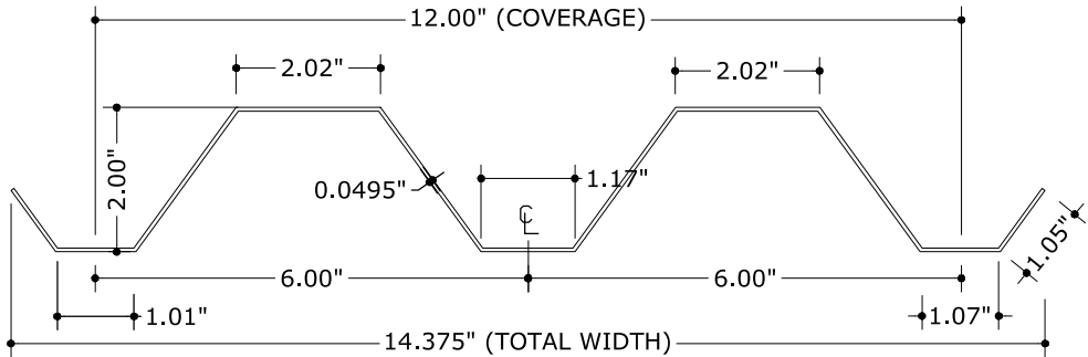
1 ALUMINUM STORM PANEL
