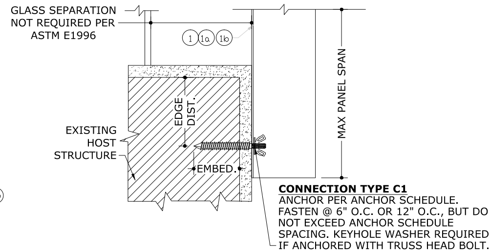
F DIRECT MOUNT SECTION
