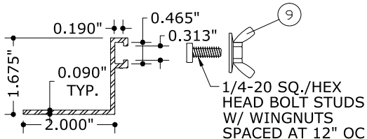
3a BUILD-OUT "U" HEADER
