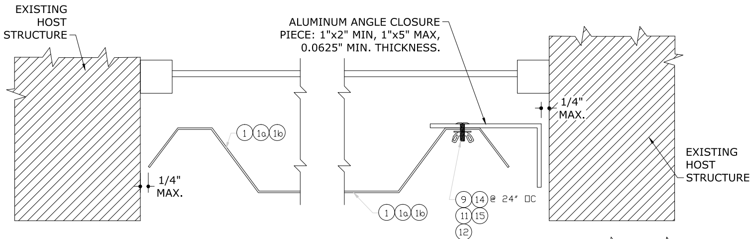
R TRAP MOUNT CLOSURE DETAIL
