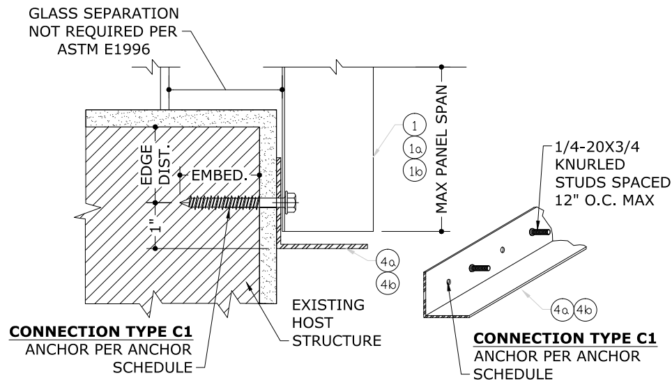
D STUD ANGLE WALL MOUNT SECTION
