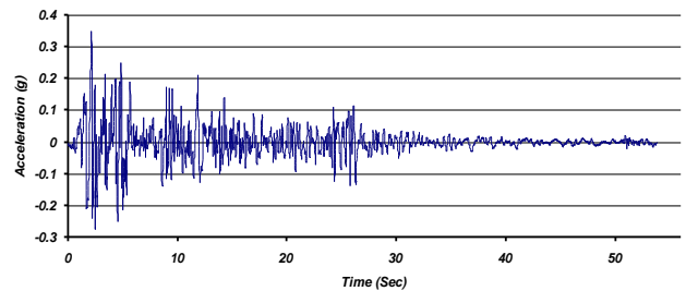
(a) El-Centro earthquake north-south direction record data graph
