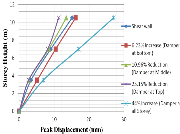
Figure 5. Peak Storey Displacements of Model Type One
