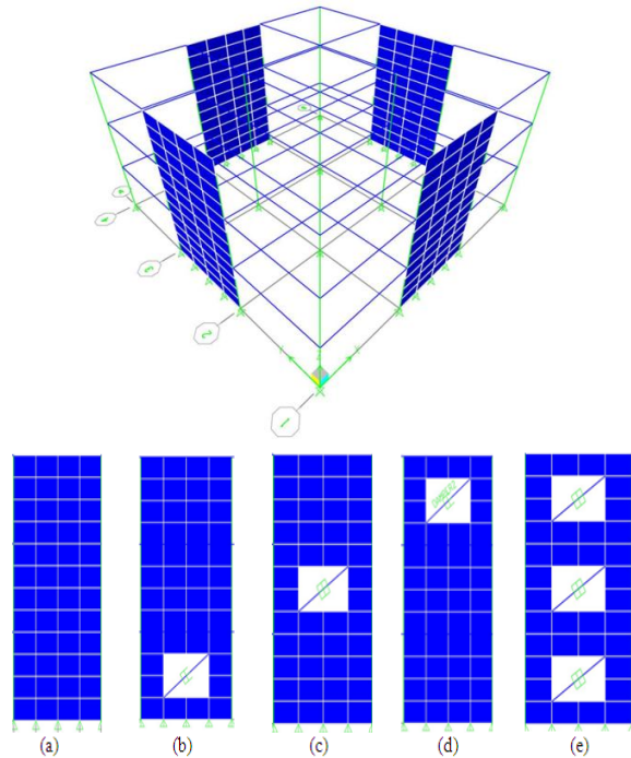
Figure 1. Model type one
