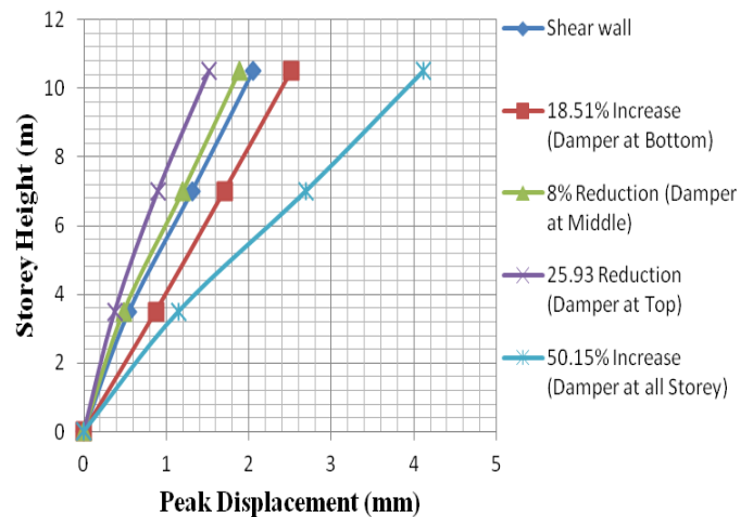
Figure 6. Peak Storey Displacements of Model Type two
