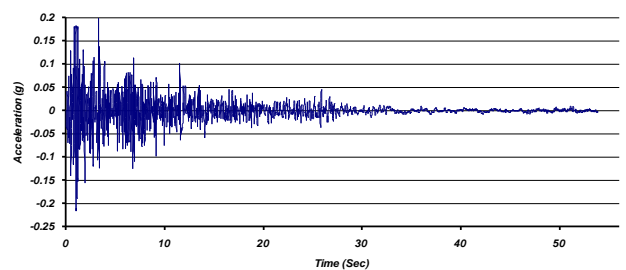
(c) El-Centro earthquake Z direction record data graph
