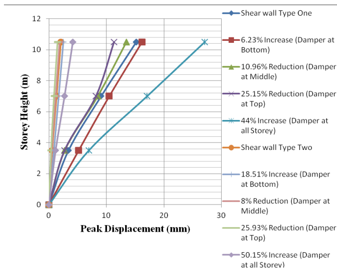
Figure7. Comparison of Peak Storey Displacements of Shear wall Type 1 and Shear wall Type 2
