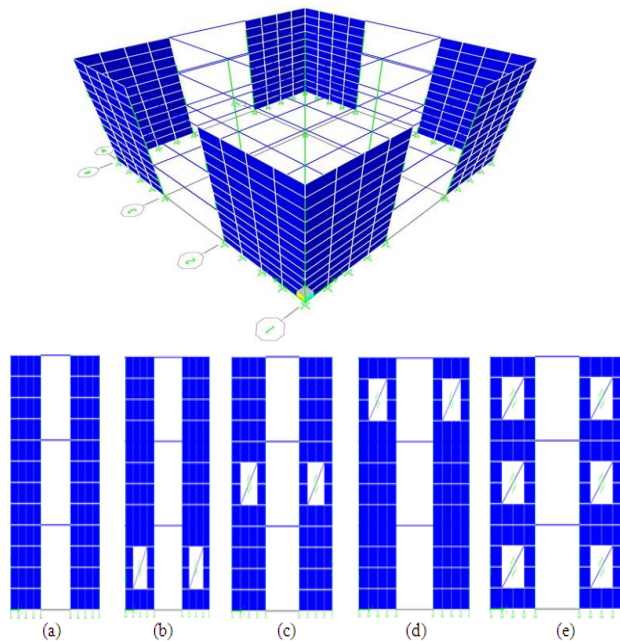
Figure 2. Model type two
