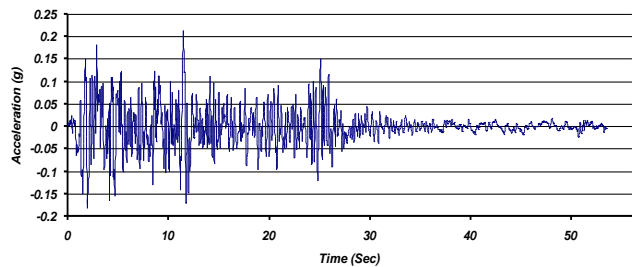
(b) El-Centro earthquake Y direction record data graph
