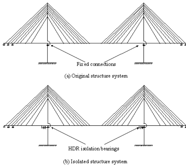
Fig. 5. Isolated system of a cable-stayed bridge model
