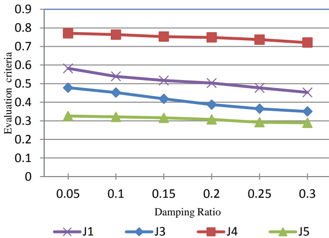
Fig. 7. Effect of damping ratio of HDR bearings on seismic response of the bridge
