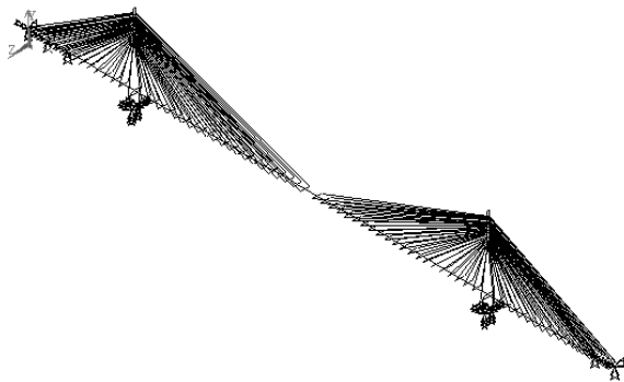
Fig. 2. Three-dimensional FE model of the Tatara cable-stayed bridge
