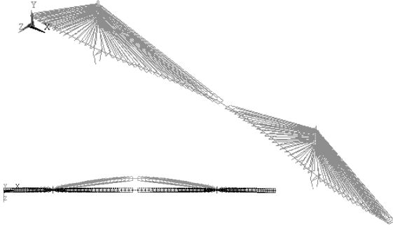
1 st Transverse bending mode (0.1326 Hz) Fig. 3. First mode shape of the FE model with fixed connections
