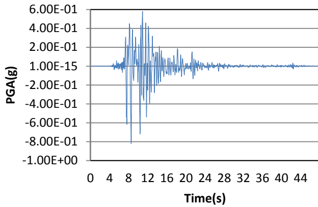
Fig. 4. Ground acceleration time-history curve of Kobe, 1995, earthquake in(longitudinal direction (N-S))
