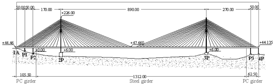
Fig. 1. General arrangement of the Tatara cable-stayed bridge
