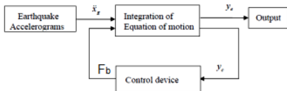
Fig. 6. The schematic process of seismic analysis of the isolation system [14]
