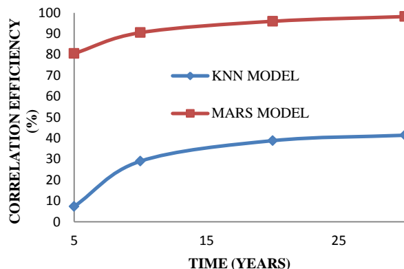
Figure 3: Relationships between CE and Length of Data Sets
