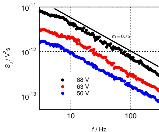
Figure 6. Low frequency noise spectral density of sample before applying the process of thermal stressing.
