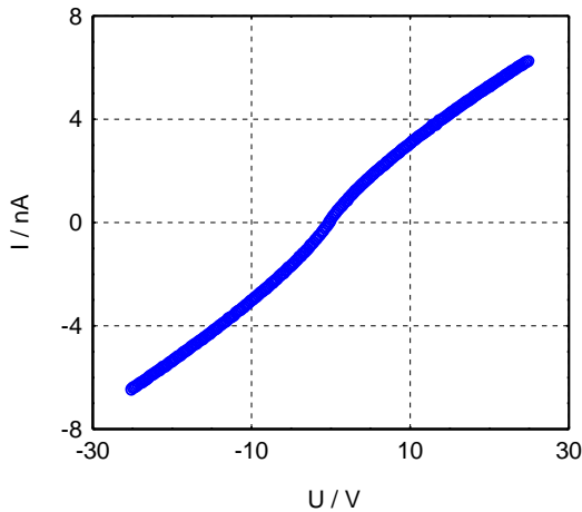
Figure 2. IV characteristic of the sample before applying the process of thermal stressing.
