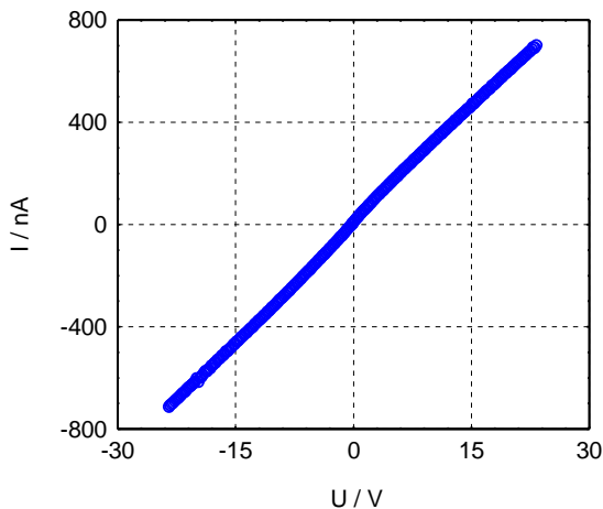
Figure 3. IV characteristic of the sample after applying the process of thermal stressing.
