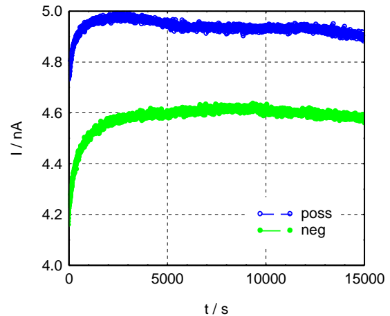
Figure 4. Current transit after detector biasing of the sample before applying the process of thermal stressing.
