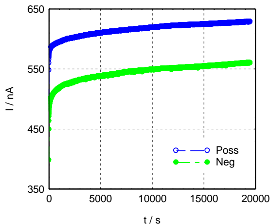
Figure 5. Current transit after detector biasing of the sample after applying the process of thermal stressing.
