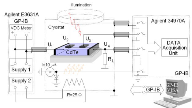
Figure 1. Experimental setup for the transport and the noise characteristics measurements.
