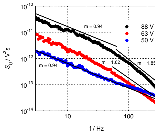
Figure 7. Low frequency noise spectral density of sample after applying the process of thermal stressing.
