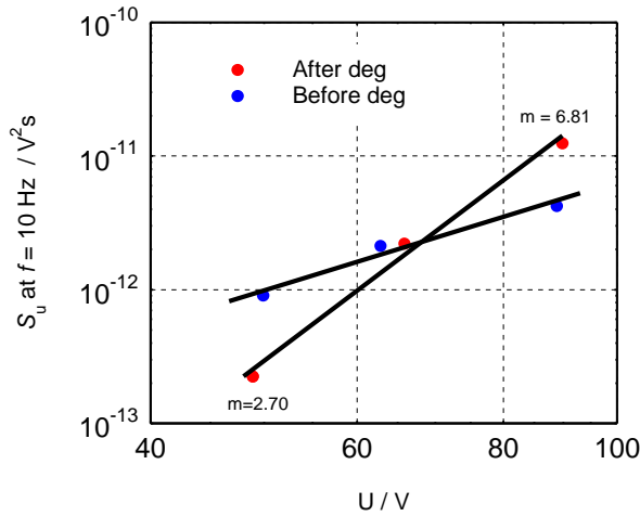
Figure 8. Low frequency noise spectral density vs. applied voltage at f = 10 Hz of the detector.
