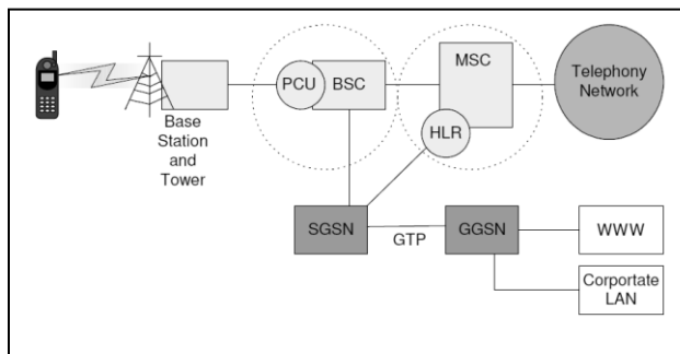
Figure2. GPRS Network Architecture
