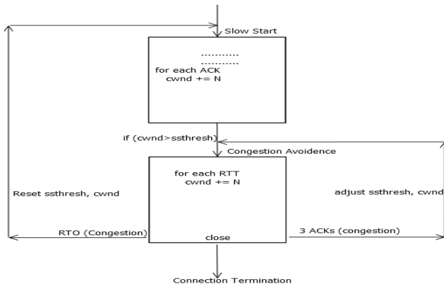
Figure 3.1: Slow Start & Congestion Avoidance Phases in TCP-RP
