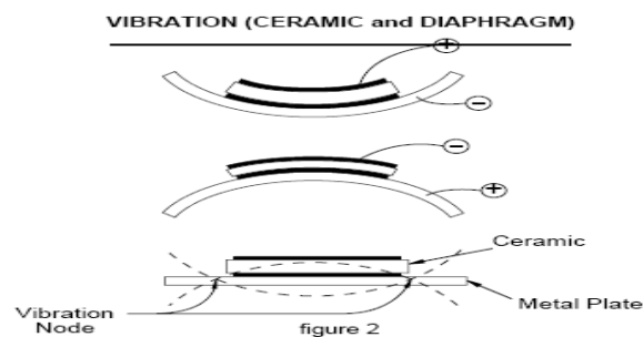
Fig 2.3vibration (ceramic &diaphragm)
