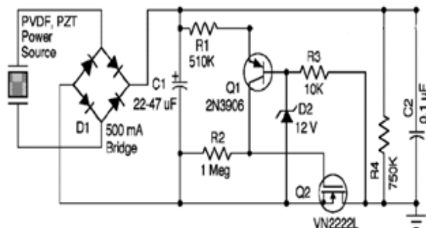
Fig 3.1 Voltage Regulation Circuit
