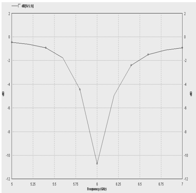
Figure 5 – Return Loss at 6 GHz
