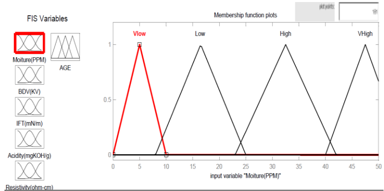
Figure 2. FIS editor showing 5-input variables and 1-output variable.
