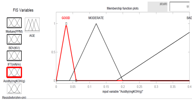
Figure 6. FIS editor membership function plot for “Acidity”.
