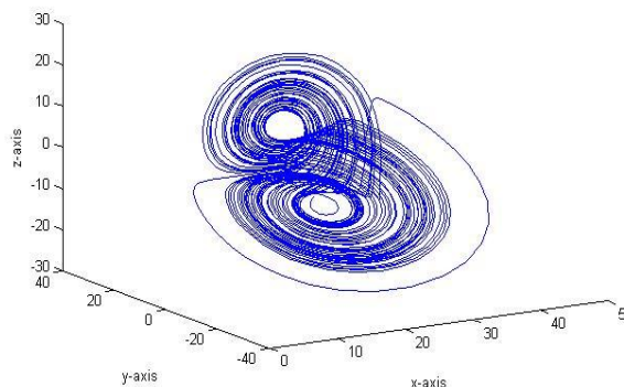
Figure 1. The new chaotic attractor when u=0
