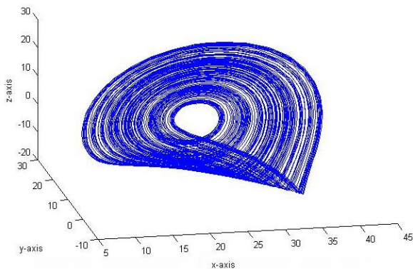
Figure 3. The new chaotic attractor when u=11
