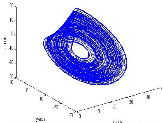
Figure 2. The new chaotic attractor when u= -11
