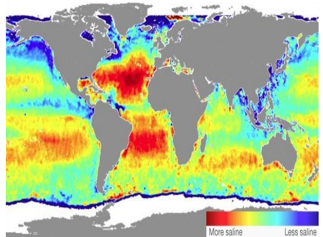
Figure 1. Ocean Salinity Satellite Image
