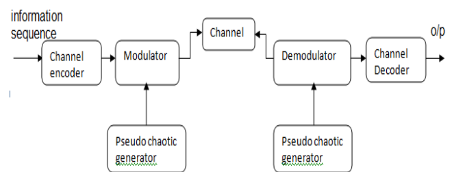
Fig.2.DS-SS block diagram
