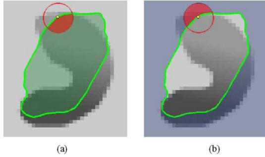
Fig. 2. Ball is considered at each point along the contour. This ball is split by the contour into local interior and local exterior regions. In both images, the point is represented by the small dot. The neighbourhood is represented by the larger red circle. In (a), the local interior is the shaded part of the circle and in (b), the shaded part of the circle indicates the local exterior.[33]
