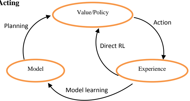
Figure 2:- Relationship among Learning, Planning and Acting.
