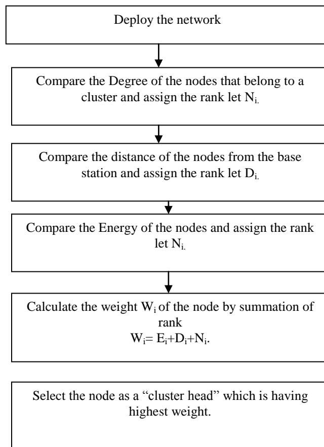
Figure 3. Data flow Diagram of Proposed approach
