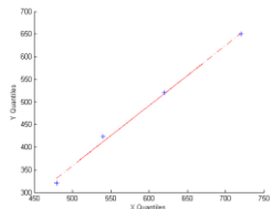
‘a1pre Vs. a1music’
