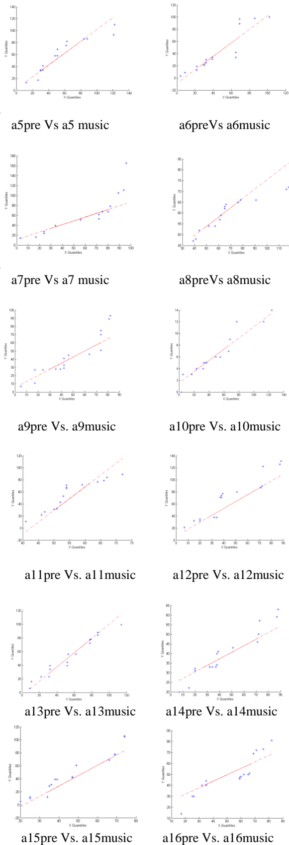
Figure 6. Q-Q plots of the rank value sequences for every pair of pre-music and on-music HRV.
