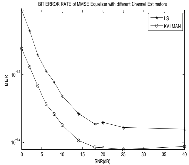
Fig3. BER performance of MMSE Equalizer with LS and KALMAN Channel Estimator
