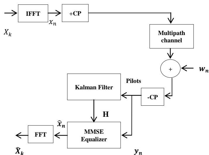
Fig 1. Block Diagram of OFDM System
