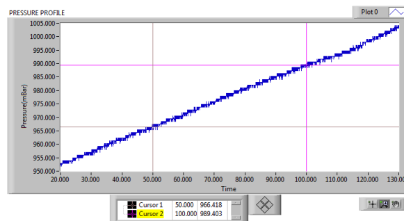
Figure 1 Pressure Profile in steady state region
