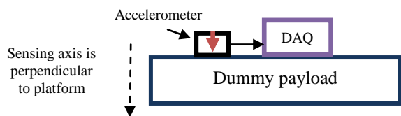
Figure 3 Accelerometer based velocity measurement setup
