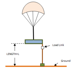
Figure 11: Load Link with mass touching ground ( T_1 )
