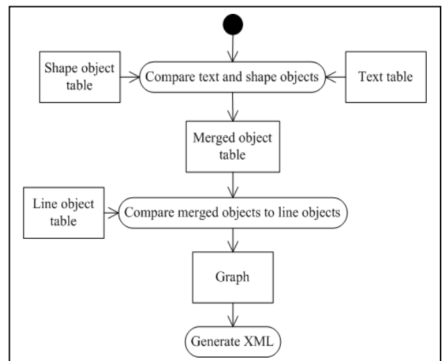
Figure 3. Match object composition procedure.
