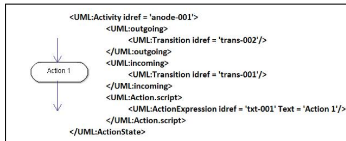
Figure 4. Action node transformed to XML.
