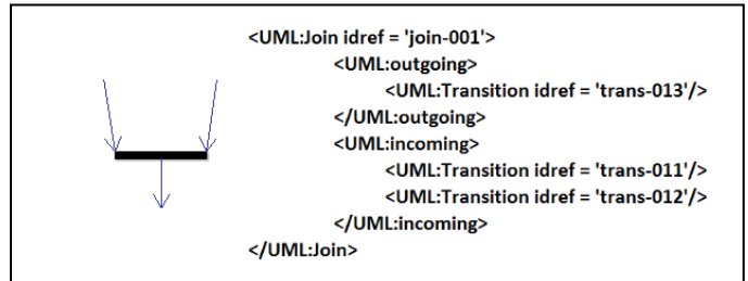
Figure 7. Join node transformed to XML.
