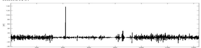
Figure 4. EEfieldiff prior to 6.6R EQ on January 6, 2008.
