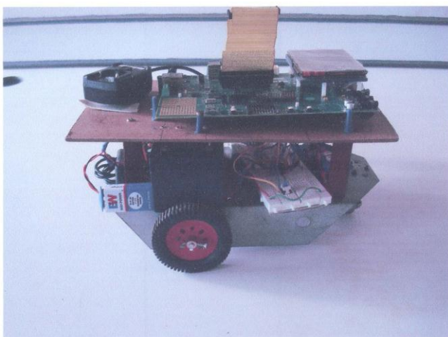
Figure 4. Side view of the prototype
