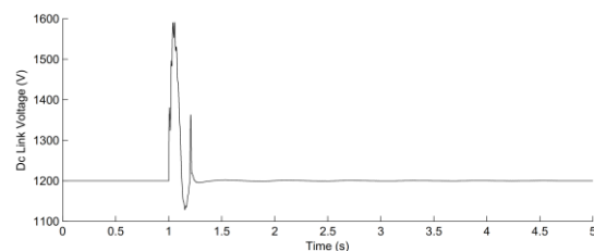
Figure 6. Dc link voltage.
