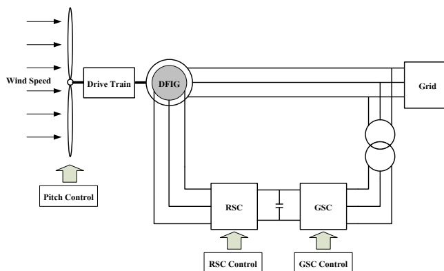
Figure 1. DFIG based on wind energy conversion system.
