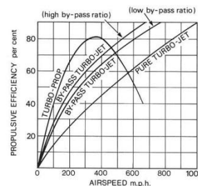
Fig 8: Propulsive efficiency comparisons between different turbojets
