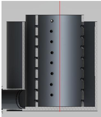
Fig4: Sectional view
