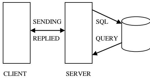
Figure 3. 2-Tier Architecture.
