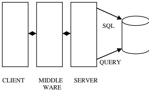
Figure 4. 3-Tier Architecture.
