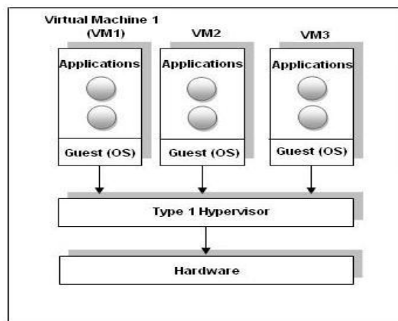
Fig. 6 Type1 Hypervisor
