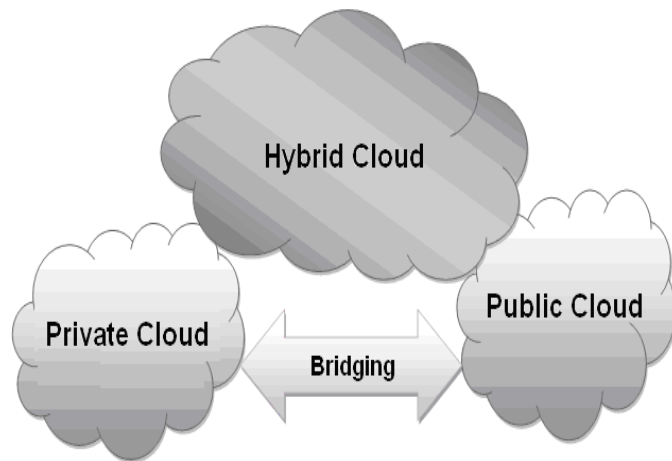
Fig. 2 Modelled Architecture
