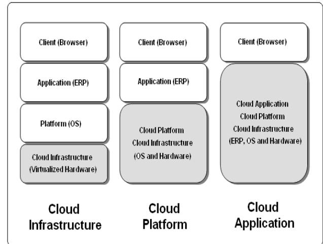
Fig. 1 Layered Architecture
