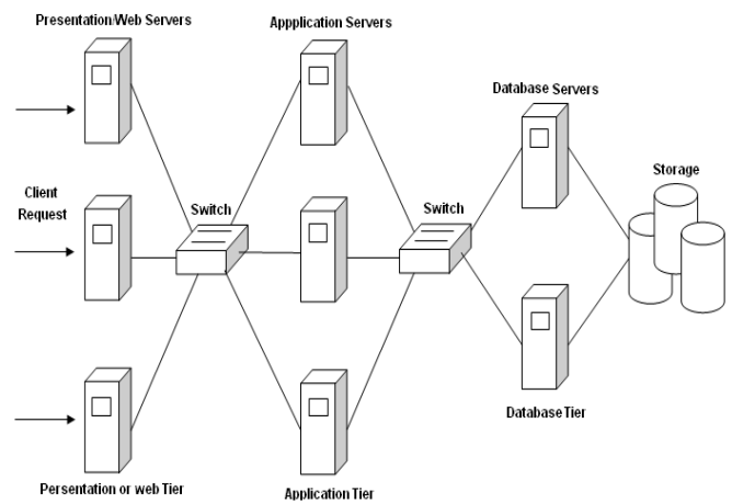
Fig. 9 Three-Tier Architecture
