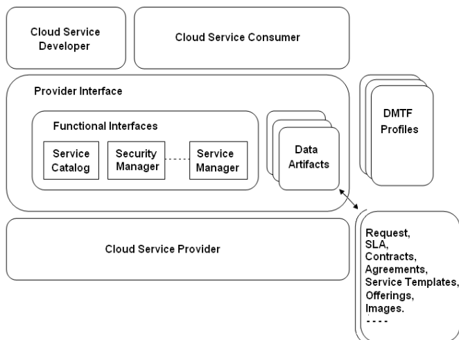
Fig. 4 DMTF Proposed Reference Architecture
