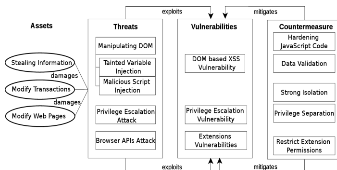
Figure 1. Threat Model for the Man-in-the-Browser Attack
