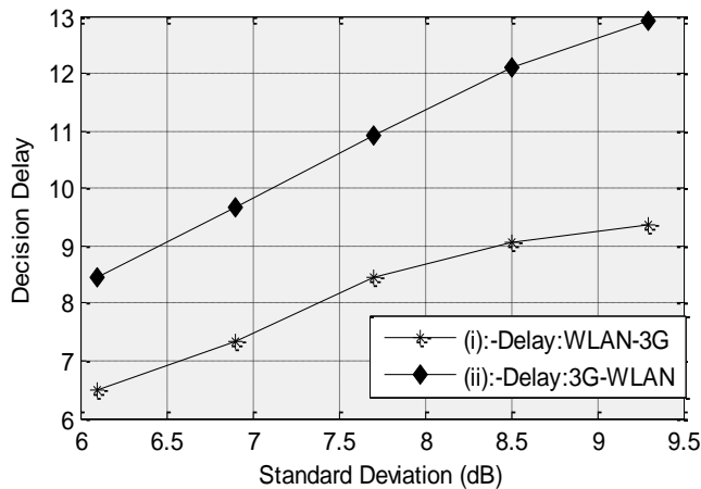
Figure 5. The decision delay vs standard deviation of shadow fading for v=5\text{m/s} , d_i = 20\text{m} and O_L = 7\text{dB}
