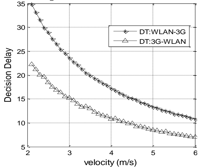
Figure 3. The decision delay vs velocity for \sigma = 8\text{dB} , d_d = 20\text{m} , and O_L = 7\text{dB} .
