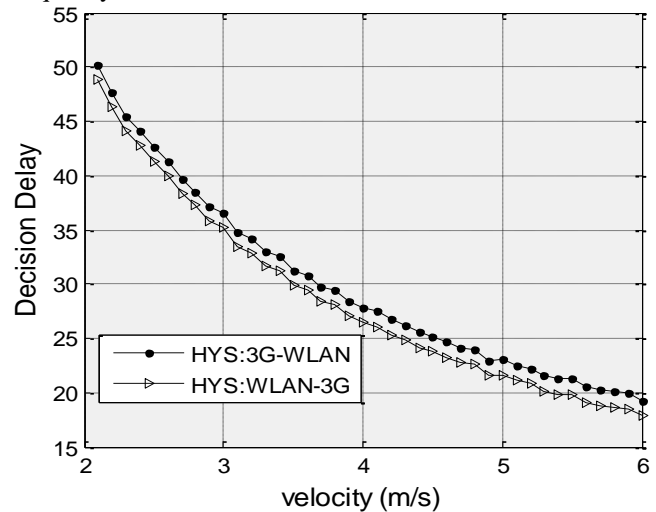
Figure 4. The decision delay vs velocity for \sigma = 8\text{dB} , d_d = 20\text{m} , and O_L = 7\text{dB} .
