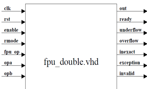
Figure 8: Top level module of Floating point unit
