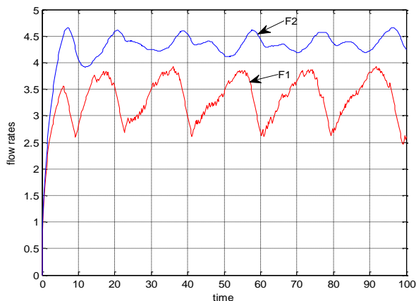
Figure 9. Flow rates of the Two Tank Liquid Level System
