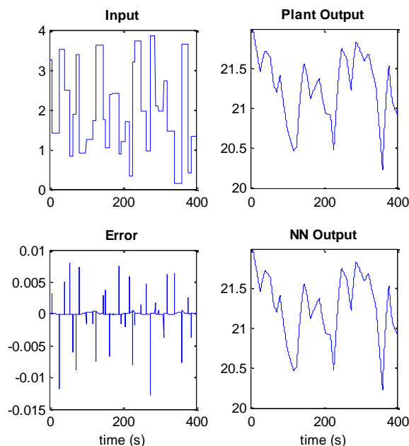
Figure 7. Validation data for NN Predictive Control
