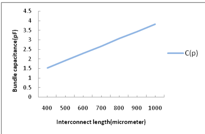
Figure 3 (c). Variation of bundle capacitance as a function of interconnect length at 32 nm technology node.
