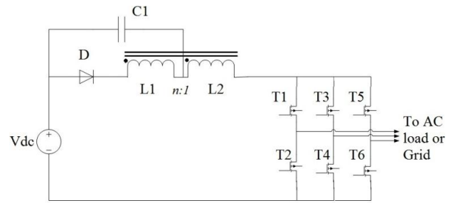
Figure 3. Voltage fed T-Shaped Z-Source Inverter.
