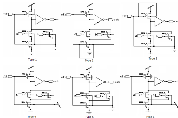
Figure1. Various Bulk Biasing techniques for Domino OR [5].
