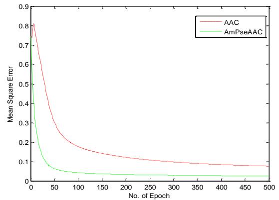
Fig. 5 Comparison of convergence characteristics of FLANN based classifier for the 277 protein domain using AAC and AmPseAAC features
