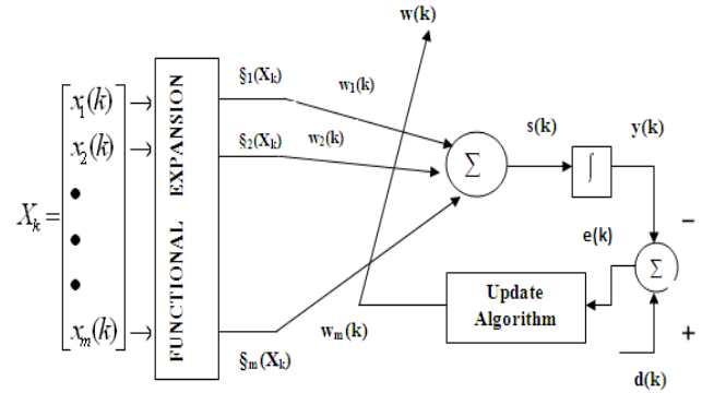
Fig.2 A simple functional link artificial neural network architecture
