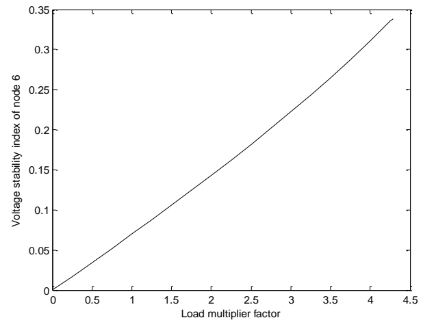
Figure 4: Voltage stability index Vs. load multiplier factor ( \alpha ) of the weakest node (node 6) of 33-node network under critical loading condition without capacitor.
