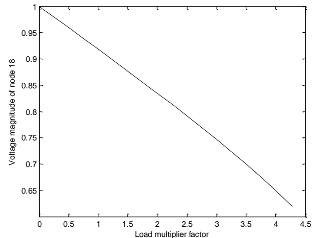
Figure 5: Voltage magnitude Vs. load multiplier factor ( \alpha ) of the weakest node (node 18) of 33-node network under critical loading condition without capacitor.
