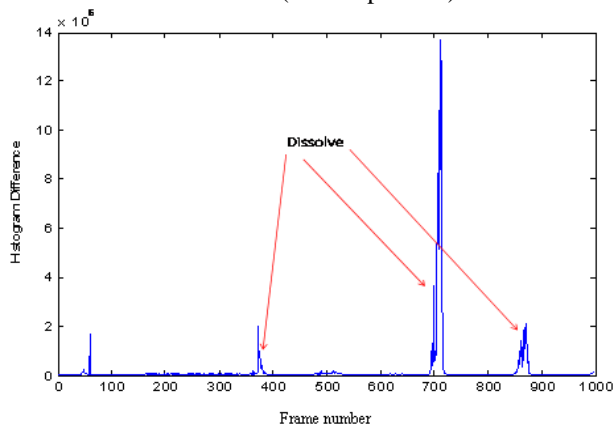
Figure. 5: Gradual boundary detection (Dissolve)
