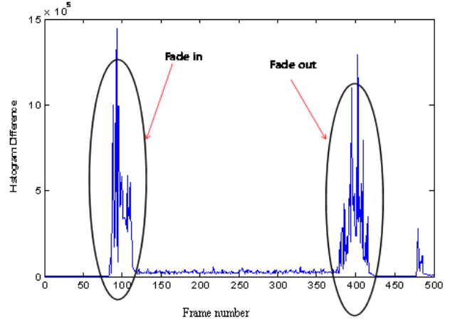
Figure.9: Gradual boundary detection (Fade)
