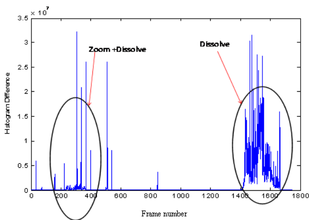
Figure 8: Gradual boundary detection (Dissolve)
