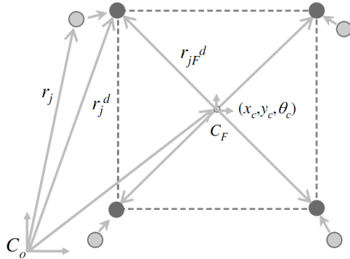
Fig.1. A formation composed of four vehicles
