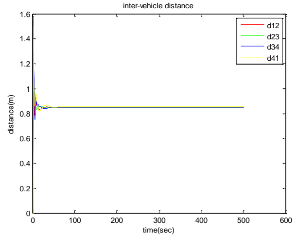
Fig.6. Inter vehicle distance within formation
