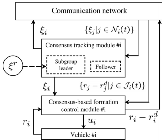
Fig.3 Formation control architecture
