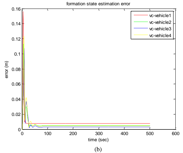
Fig. 5: (a) vehicle trajectory, (b) formation state estimation error (vc-virtual centre)
