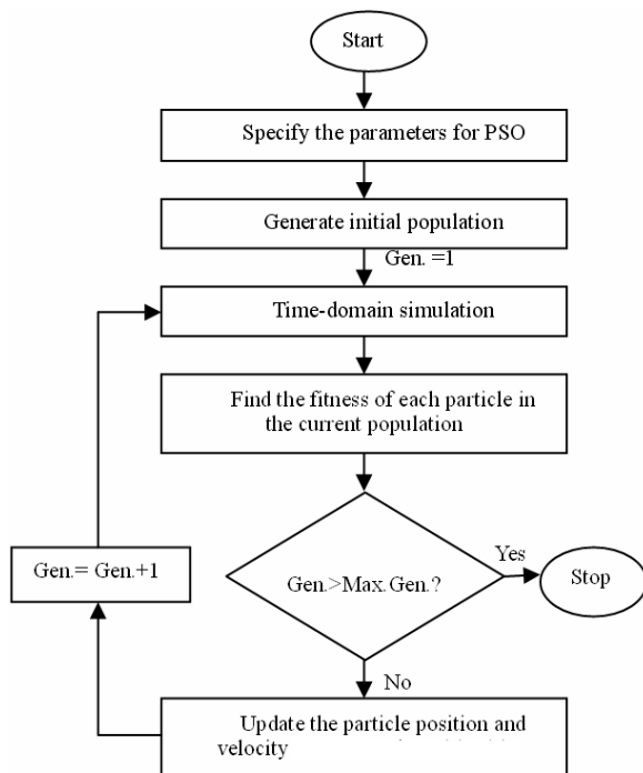
Figure 2. Flow Chart of PSO
