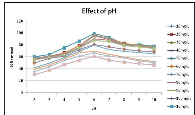
Figure 1. Effect of pH on the removal of MY dye
