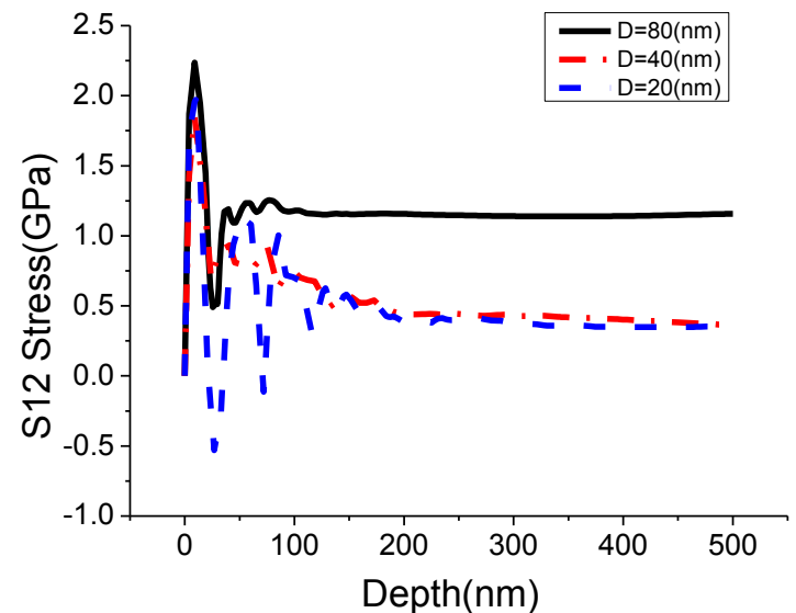
Figure 7. Shear stress variation for different inclusion size
