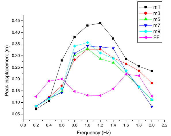
Figure 7: Variation of displacement response spectra with cluster size for nine storied building group, at edge of cluster.
