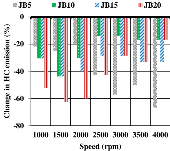
Fig. 5 Change in HC emission (%) of different blends of Jatropha biodiesel compared to diesel combustion
