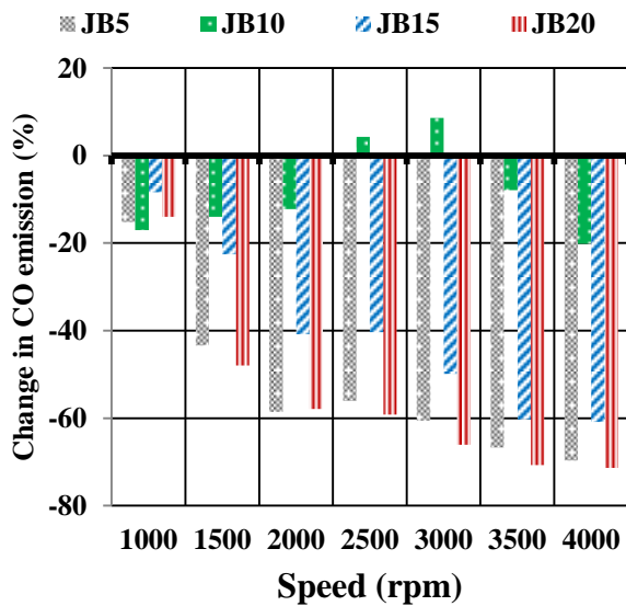
Fig. 6 Change in CO emission (%) of different blends of Jatropha biodiesel compared to diesel combustion.
