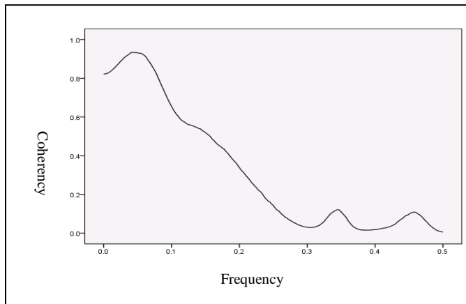
Figure 2. Coherence spectrum of wind speed and wave height for Platform-A in the month of August 1999
