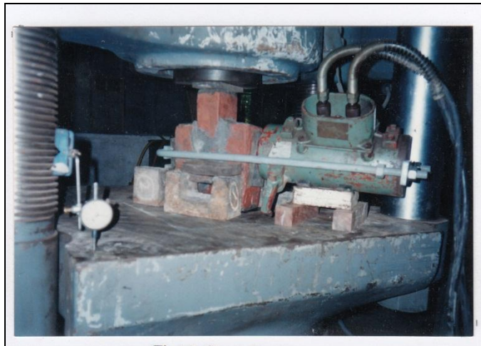
Figure 2. Shear test Setup
